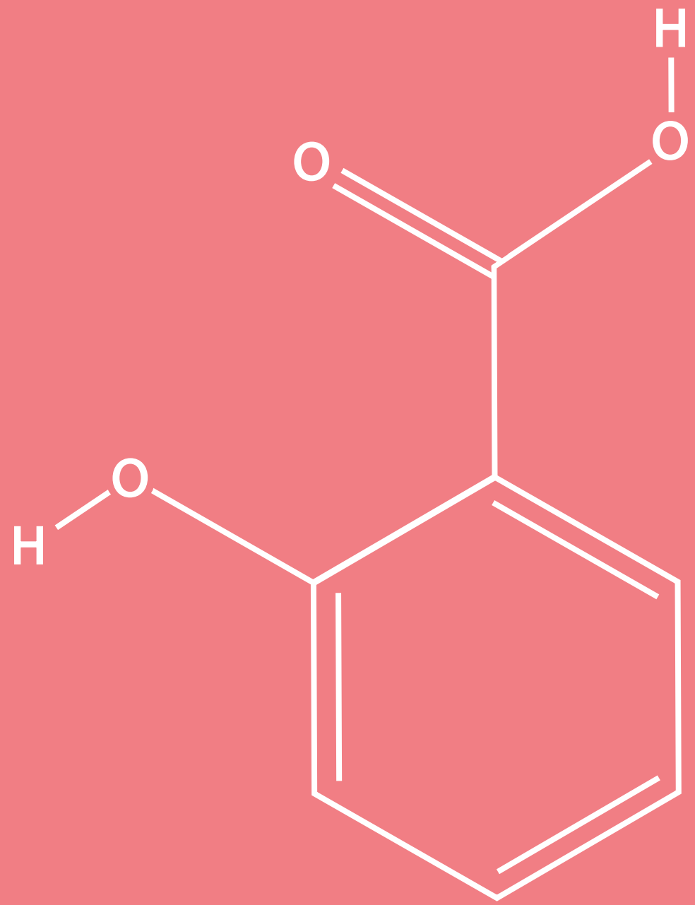
Skeletal Formula
